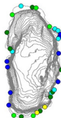
Figure 6.5.4.2.3.1-1 Trophic state of the littoral zone of Lake Ohrid, based on the macrophyte index of Melzer (1999) and Melzer and Schneider (2001). Areas with low population density generally show oligotrophic to oligo-mesotrophic conditions while the more densely populated areas on the south and north shores show mesotrophic to meso-eutrophic conditions. Source: Christiansen et al. (2013).
