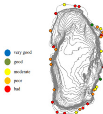
Figure 6.5.4.3.3.1-1 Ecological status of the littoral zone of Lake Ohrid based on the Intercalibration Common Metric (ICM) for the Central-Baltic Ecoregion. The majority of the sites in Albania along the west and south shores showed poor to bad conditions. Moderate to good conditions were found only along the east and north shores, i.e. mainly in Macedonia (Christiansen et al. 2013).
