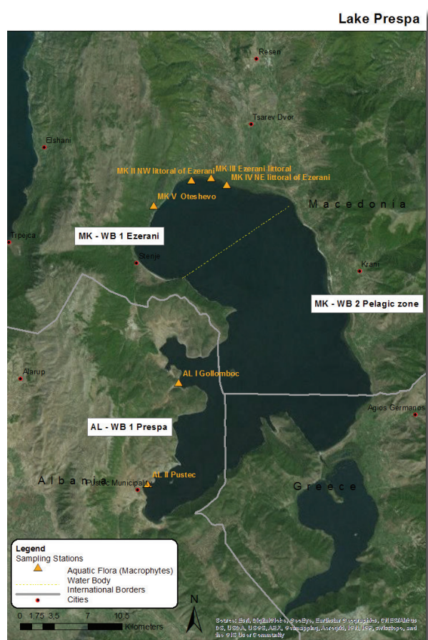
Figure 7.5.4.2.1-1 Sampling stations for macrophyte investigations at Lake Prespa Samples were taken along transects perpendicular to the shoreline.
