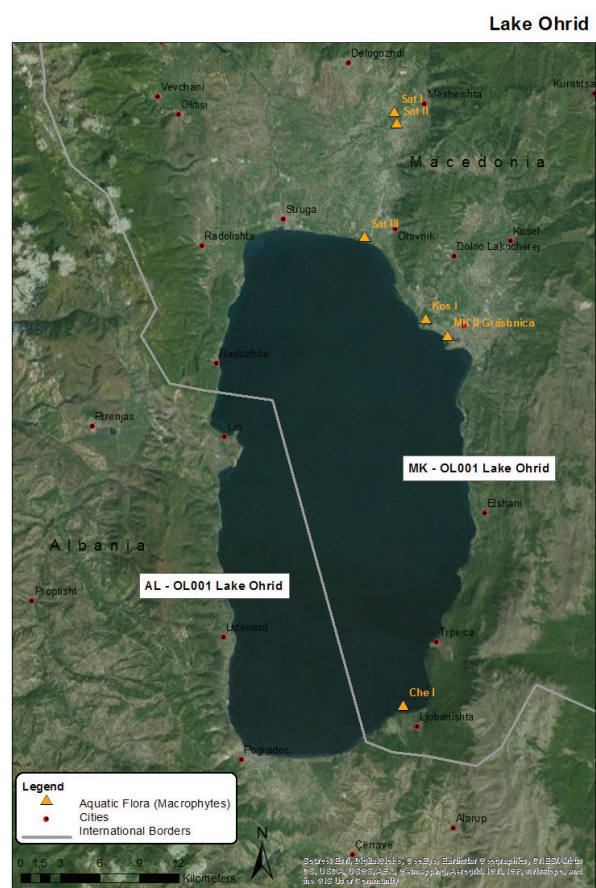
Figure 6.5.4.2.1-1 Sampling stations for macrophyte investigations at Lake Ohrid tributaries in Macedonia. All rivers were sampled at the inflow into the lake and River Sateska was also sampled upstream. No samples were collected from the Albanian part of the lake.
