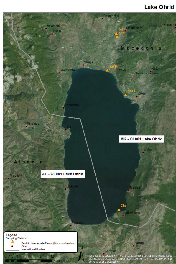
Figure 6.5.4.3.1-1 Sampling stations for macroinvertebrate investigations at Lake Ohrid tributaries in Macedonia. All rivers were sampled at the inflow into the lake while River Sateska was also sampled upstream. No samples were taken from the Albanian part of the lake.
