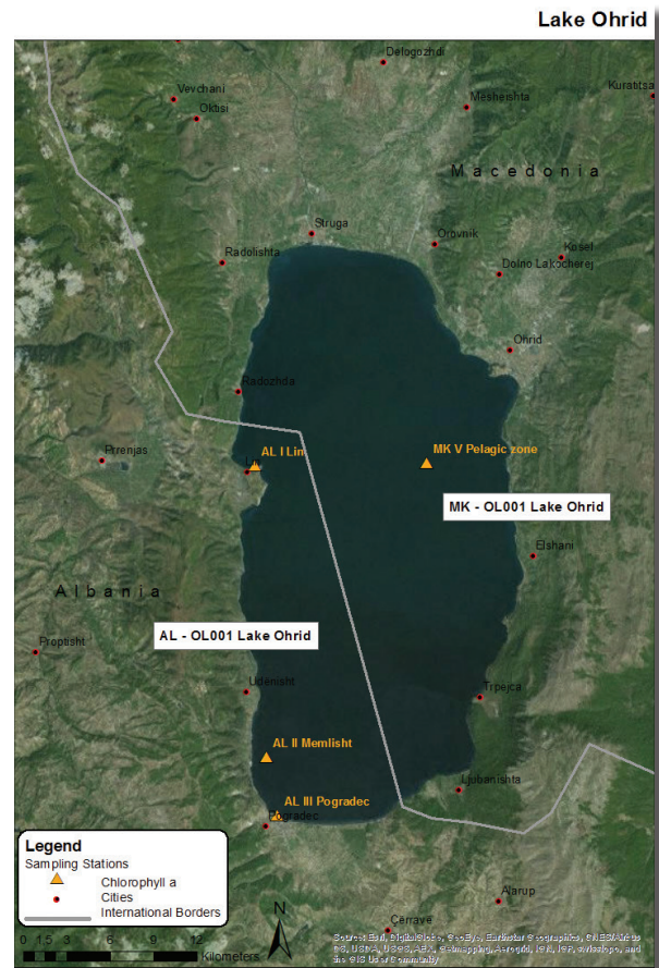
Figure 6.5.4.1.1-1 Sampling stations for chlorophyll- a analysis in Lake Ohrid. In Macedonia, samples were taken at one pelagic station from 9 depth strata. In Albania, samples were taken at three littoral stations from the upper depth stratum.
