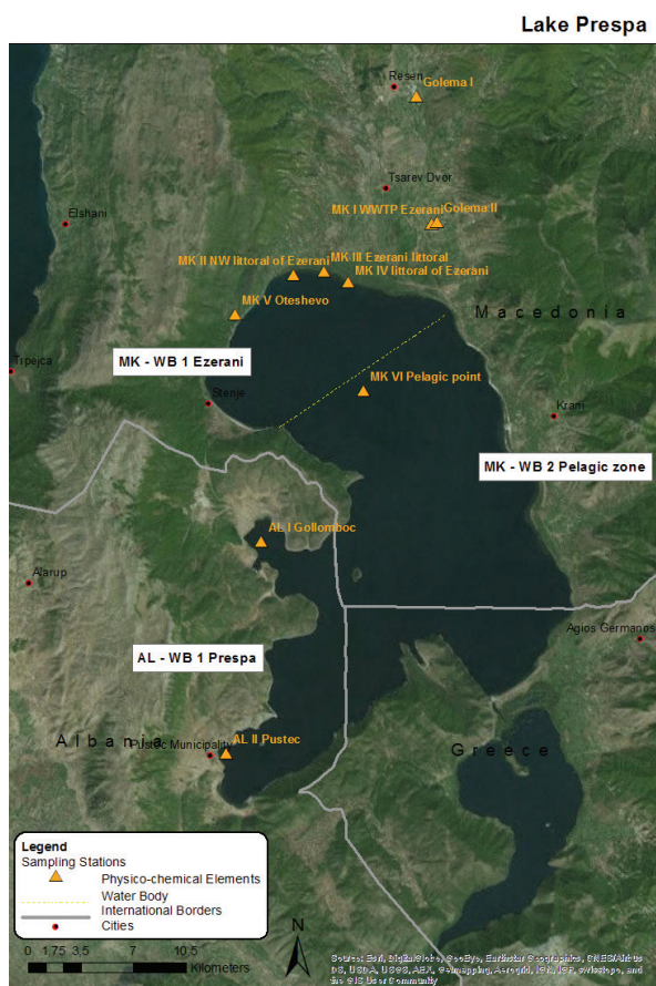
Figure 7.5.1-1 Sampling stations for chemical and physico-chemical analyses at Lake Prespa. The Technical Working Group – WFD tentatively divided Macro Prespa into three water bodies: two in Macedonia and one in Albania.
